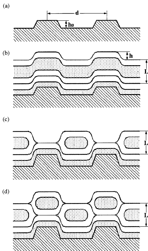
Figure 6. Schematic cross section of the configurations: (a) bare Si grating, (b) conformal arrangement of a diblock copolymer lamellar on a grating with h_0 < h_c ; (c) anticonformal configuration of a copolymer film on a grating with h > h_c ; (d) arrangement of different layers in the anticonformal case. This drawing is based on the TEM image shown in Figure 8c. Note that the uppermost two layers are anticonformal to each other.
