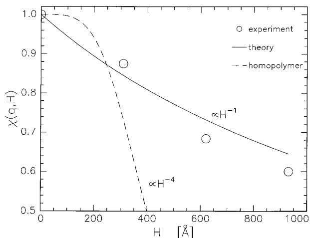
Figure 10. Measured roughness attenuation (open circles) and calculation (solid line) with the model presented in the text. The broken line is the calculation for a homopolymer liquid.
