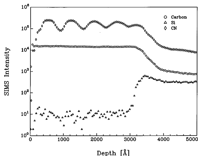
Figure 2. SIMS profiles of CN, C, and Si perpendicular to the surface from a H = 3200 Å thick N_{PS} - N_{P2VP} = 1000 - 1000 film on a Si grating with height h_0 = 250 Å.
