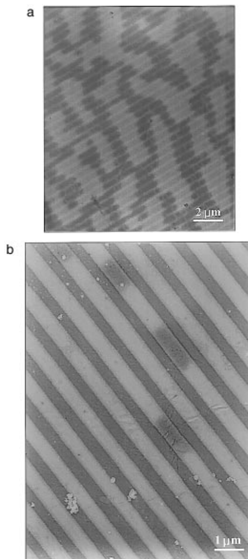
Figure 7. TEM plan view of an N_{PS} - N_{P2VP} = 1000-1000 film of thickness H \approx 710 Å on (a) a grating of h_0 = 173 Å, d = 0.5 μm, which is conformal to the grating surface and (b) a grating of h_0 = 440 Å, d = 1 μm, which is anticonformal to the grating surface.
