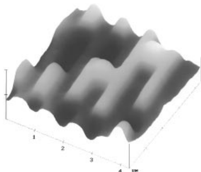
Figure 5. Three-dimensional AFM image of a N_{PS} - N_{P2VP} = 200-200 diblock copolymer film of thickness H = 660 Å on a Si grating with h_0 = 250 Å. Several layers are visible which form alternating conformal and anticonformal structures relative to the grating.
