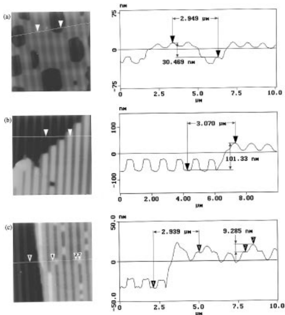
Figure 3. (a) Conformal configuration of a N_{PS} - N_{P2VP} = 200-200 PS-P2VP diblock copolymer film of total thickness H = 440 Å on grating with height h_0 = 120 Å. (b) Anticonformal configuration of a N_{PS} - N_{P2VP} = 1000-1000 film with a thickness of H = 710 Å \approx L on a grating with h_0 = 440 Å. (c) Anticonformal configuration of a N_{P2VP} - N_{PS} - N_{P2VP} = 90-560-90 triblock copolymer film of total thickness H = 400 Å on a grating with h_0 = 120 Å. The associated cross-sectional AFM scans are shown above all pictures.
