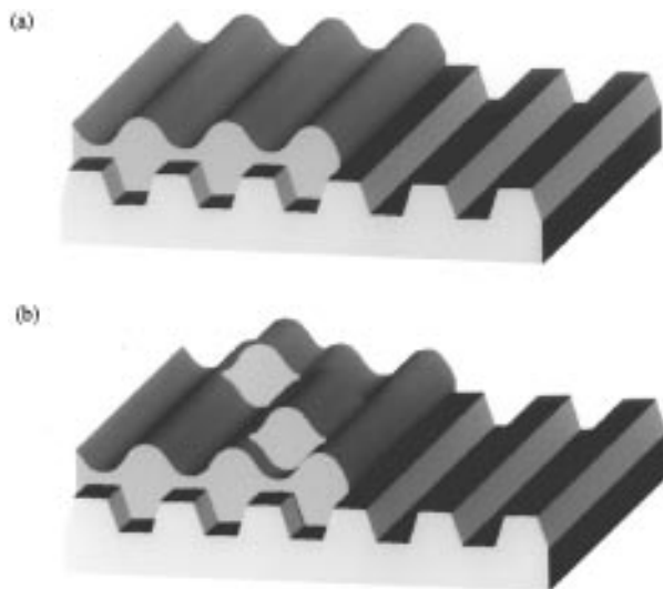
Figure 4. Schematic drawing of the anticonformal arrangement of block-copolymer films on a grating as observed by AFM in parts b and c of Figure 3.
