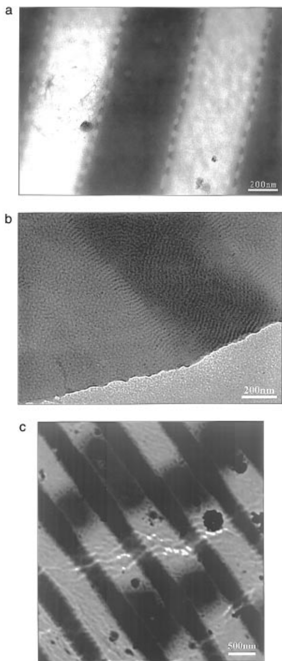
Figure 8. (a) Magnified section of the boundary at the island formed in the grating grooves shown in Figure 7b. Note the defects decorating the island boundary. (b) Ordering of cylinders in a triblock copolymer of P2VP-PS-P2VP on a grating with h_0 = 90 Å. The structure is anticonformal. (c) Plan view of a thicker edge of the film shown in Figure 7b. A third layer is seen to form in the grooves of the second. Defects decorate the boundaries of all islands.
