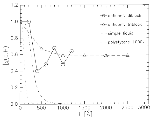
Figure 9. Roughness attenuation |\chi(q, H)| = h/h_0 as a function of the total film thickness H for different systems: small molecule liquid (dots); homopolymer liquid (broken line); diblock copolymer anticonformal case (open circles); triblock copolymer anticonformal case (open triangles). The solid and broken lines for the block copolymer films are just lines drawn to connect the points for clarity. They are not given by the theory.
