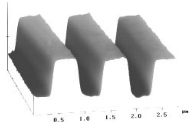
Figure 1. AFM image of a Si surface grating with periodicity d = 1 \mu\text{m} and height h_0 = 250 \text{ \AA} .
